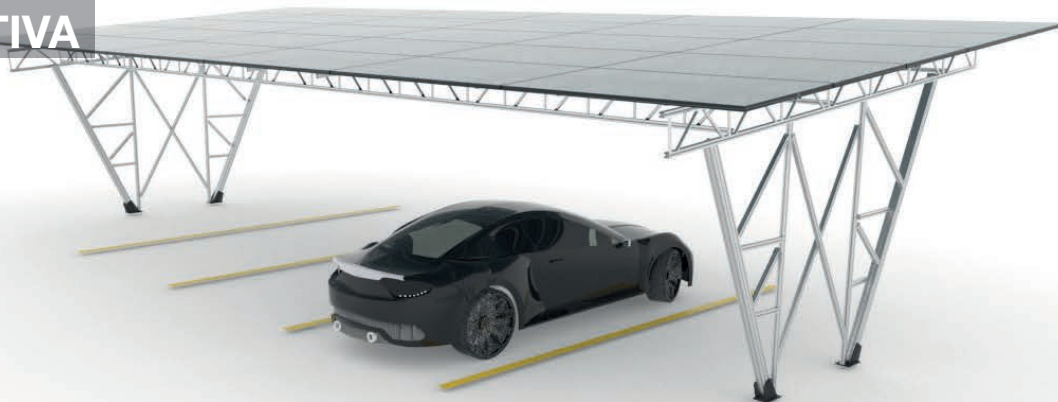
VISTA SEMI-SUPERIOR
